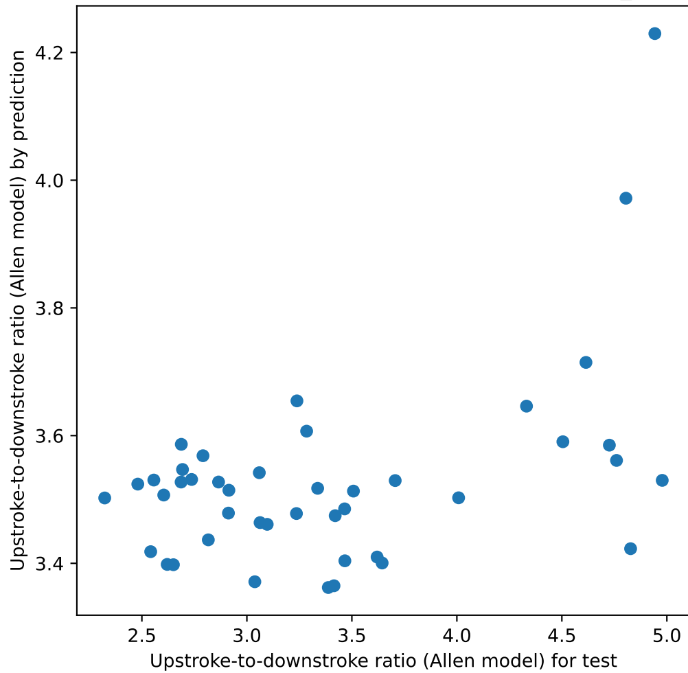
prediction of Upstroke-to-downstroke ratio (Allen model) by embs alpha 0.05 l1_ratio 0.05 positive False MAE 0.615
